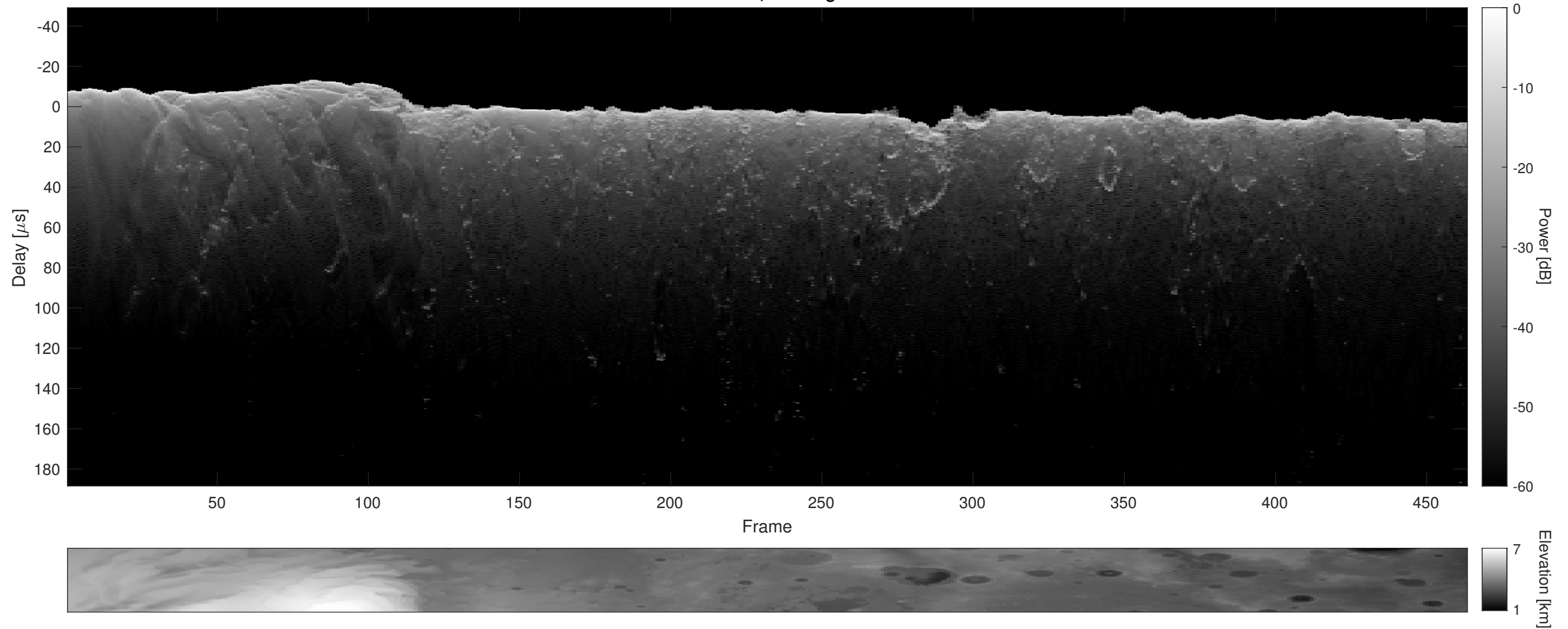
Orbit 16838, Cluttergram
