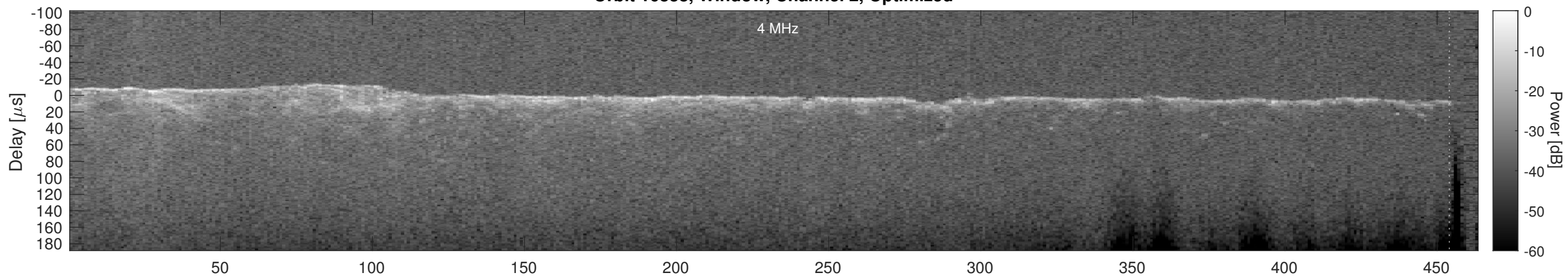
Orbit 16838, Cluttergram
