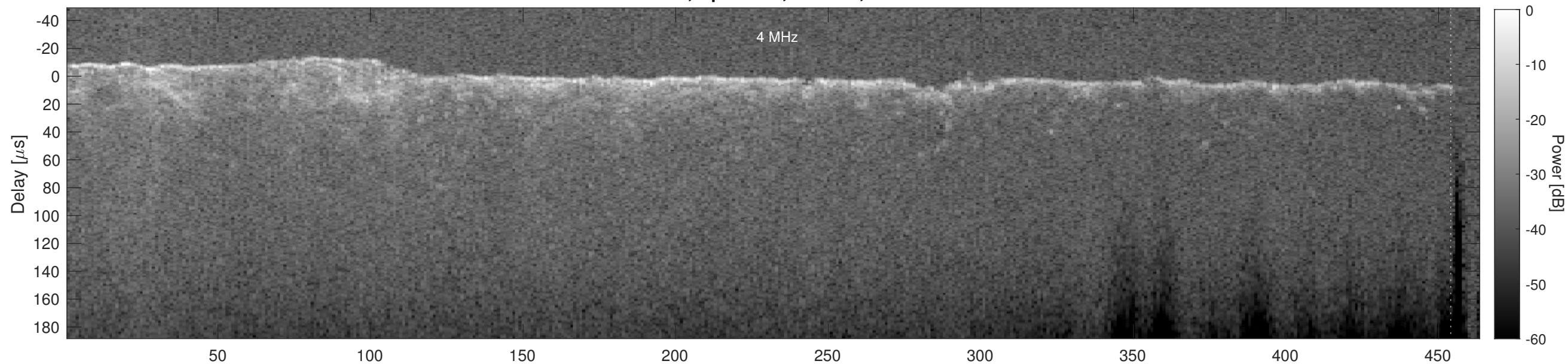
Orbit 16838, Cluttergram
