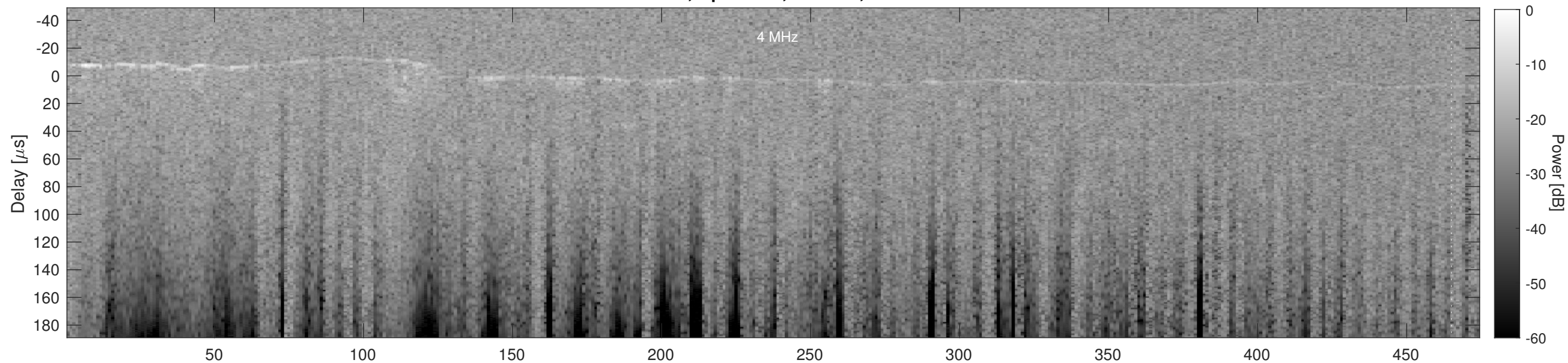
Orbit 16845, Cluttergram
