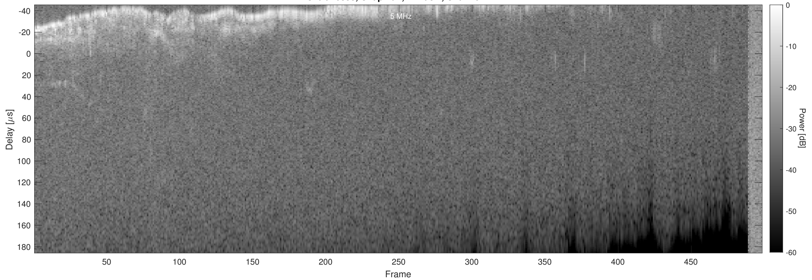
Orbit 16853, Chapman, Window, Channel 2
