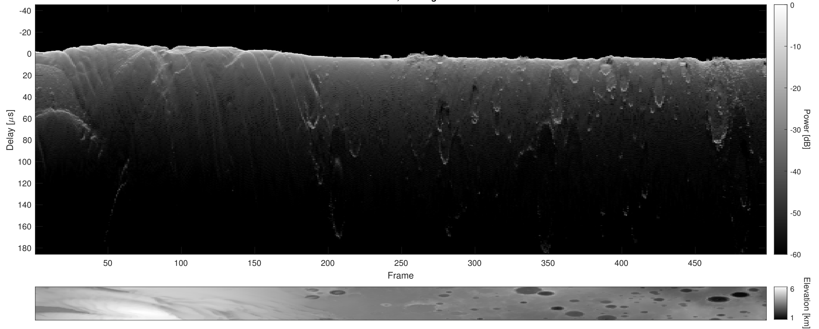
Orbit 16853, Cluttergram
