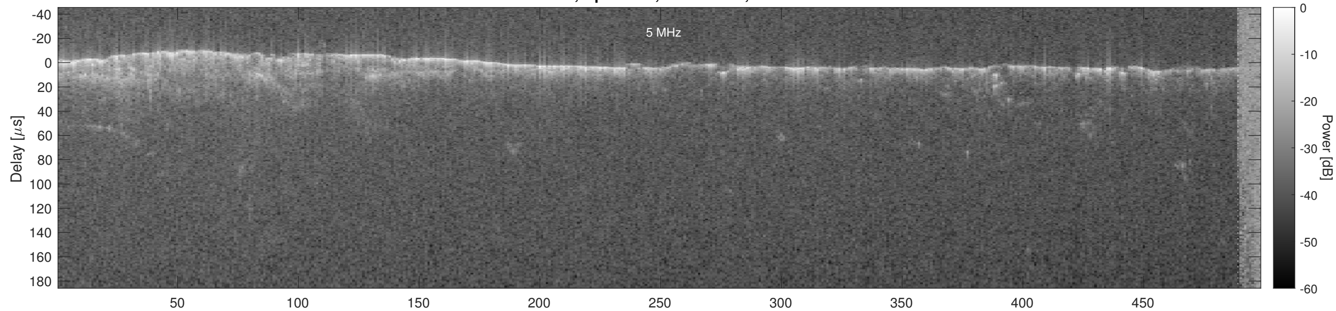
Orbit 16853, Optimized, No Window, Channel 2
