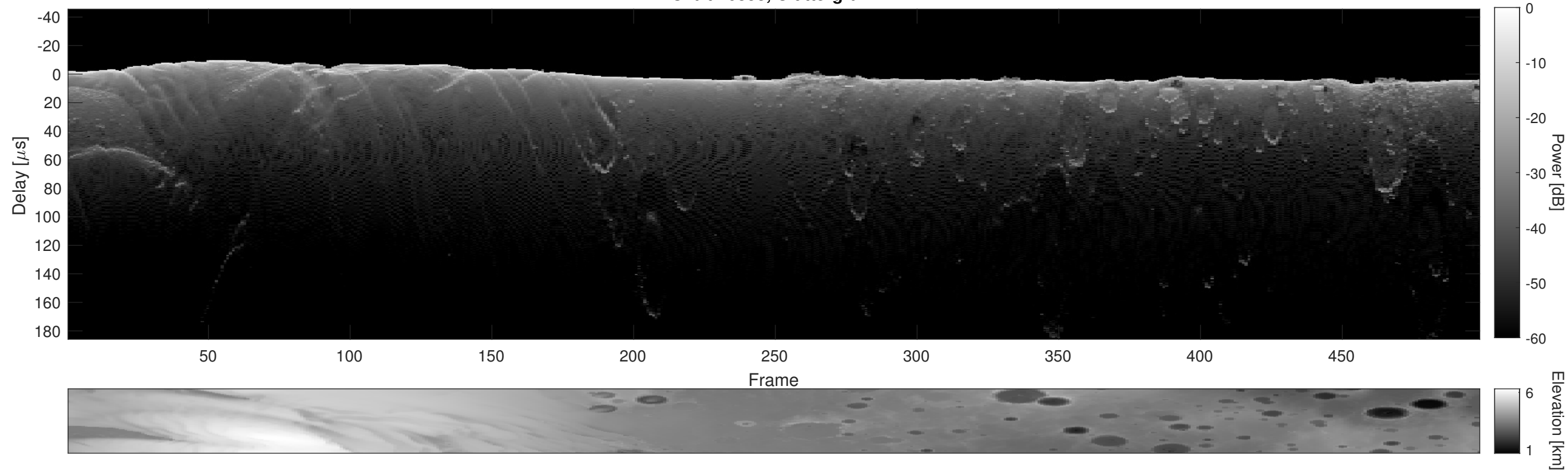
Orbit 16853, Cluttergram
