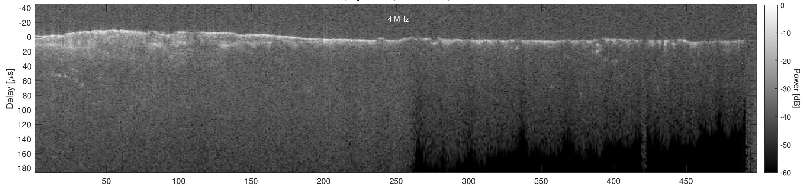
Orbit 16853, Cluttergram
