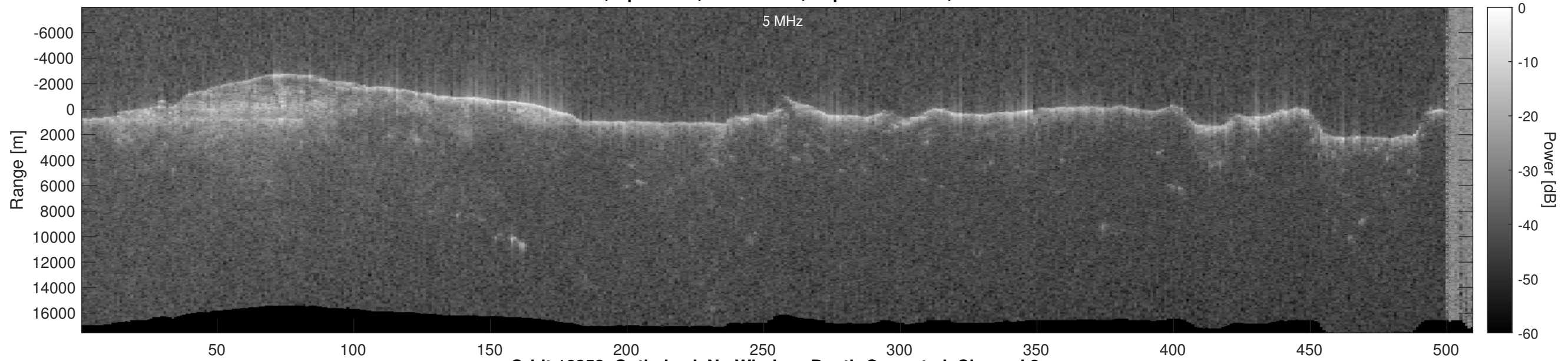
Orbit 16858, Optimized, No Window, Depth-Corrected, Channel 2
