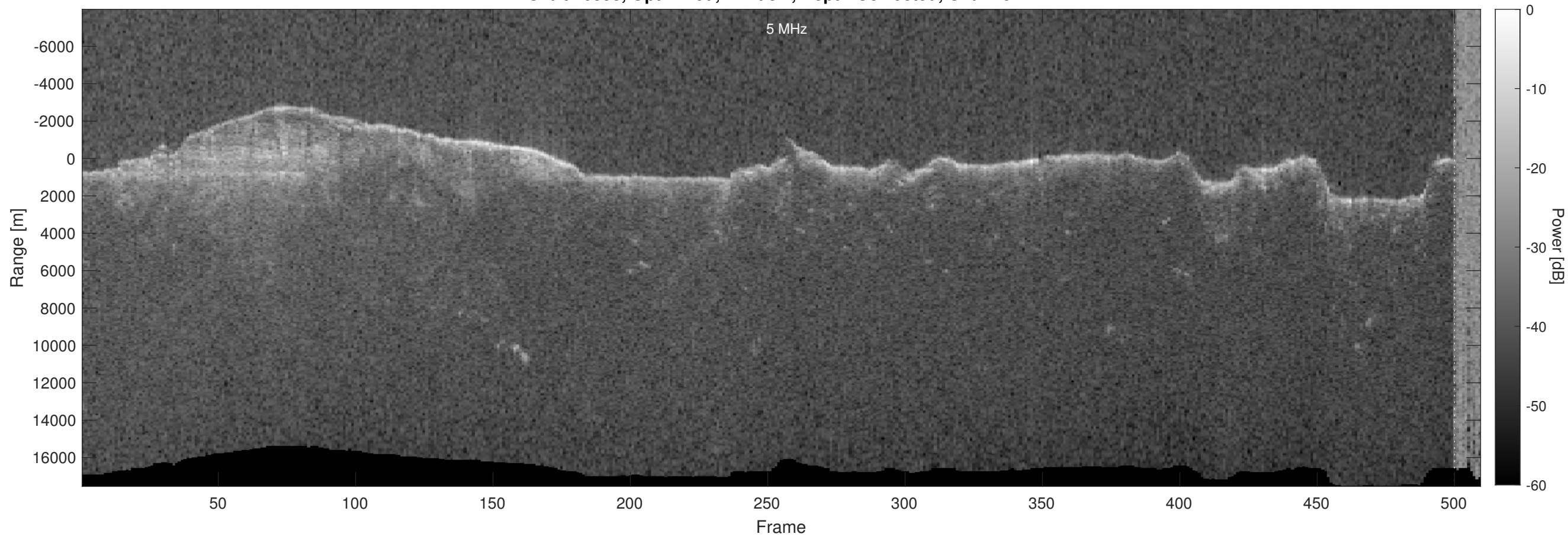
Orbit 16858, Optimized, Window, Depth-Corrected, Channel 2
