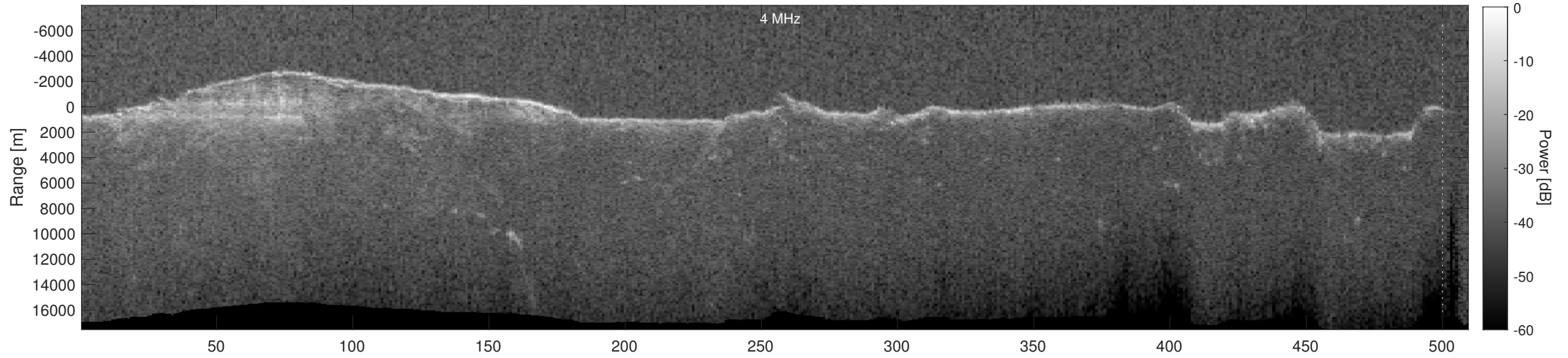
Orbit 16858, Depth-Corrected Cluttergram
