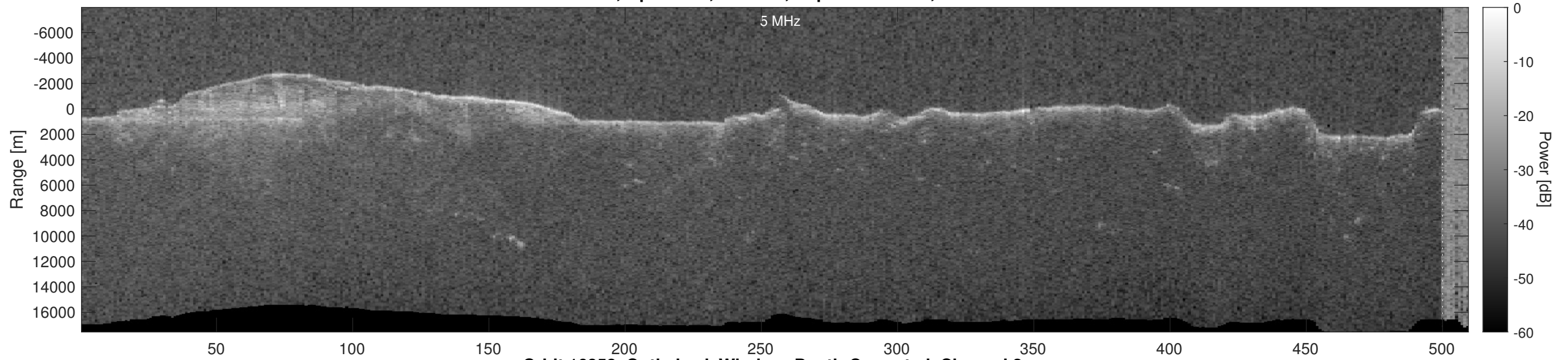
Orbit 16858, Optimized, Window, Depth-Corrected, Channel 2
