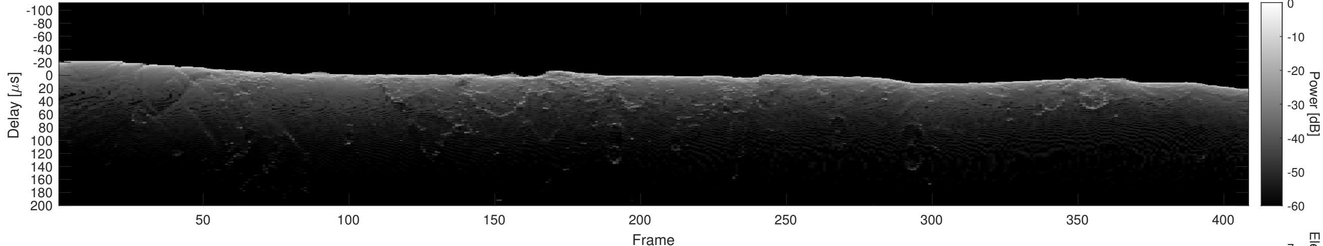
Orbit 16862, Cluttergram
