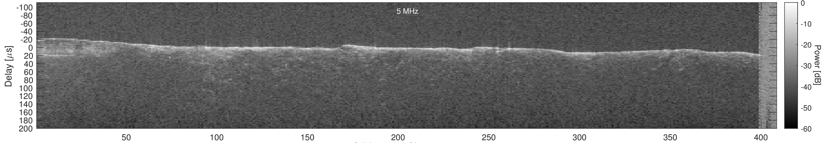
Orbit 16862, Cluttergram
