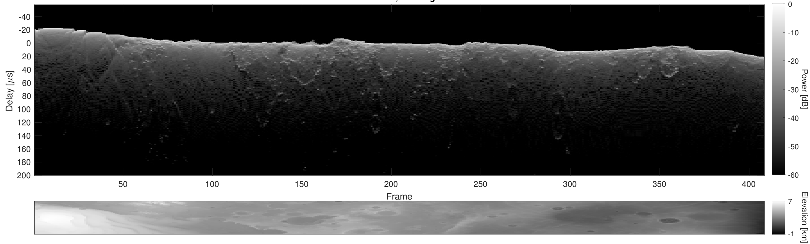
Orbit 16862, Cluttergram
