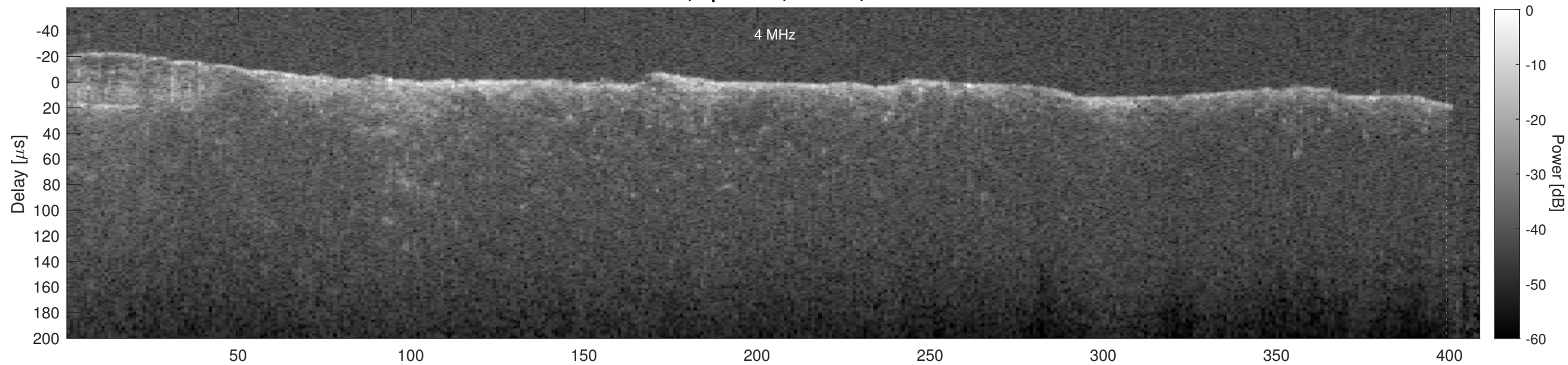
Orbit 16862, Cluttergram
