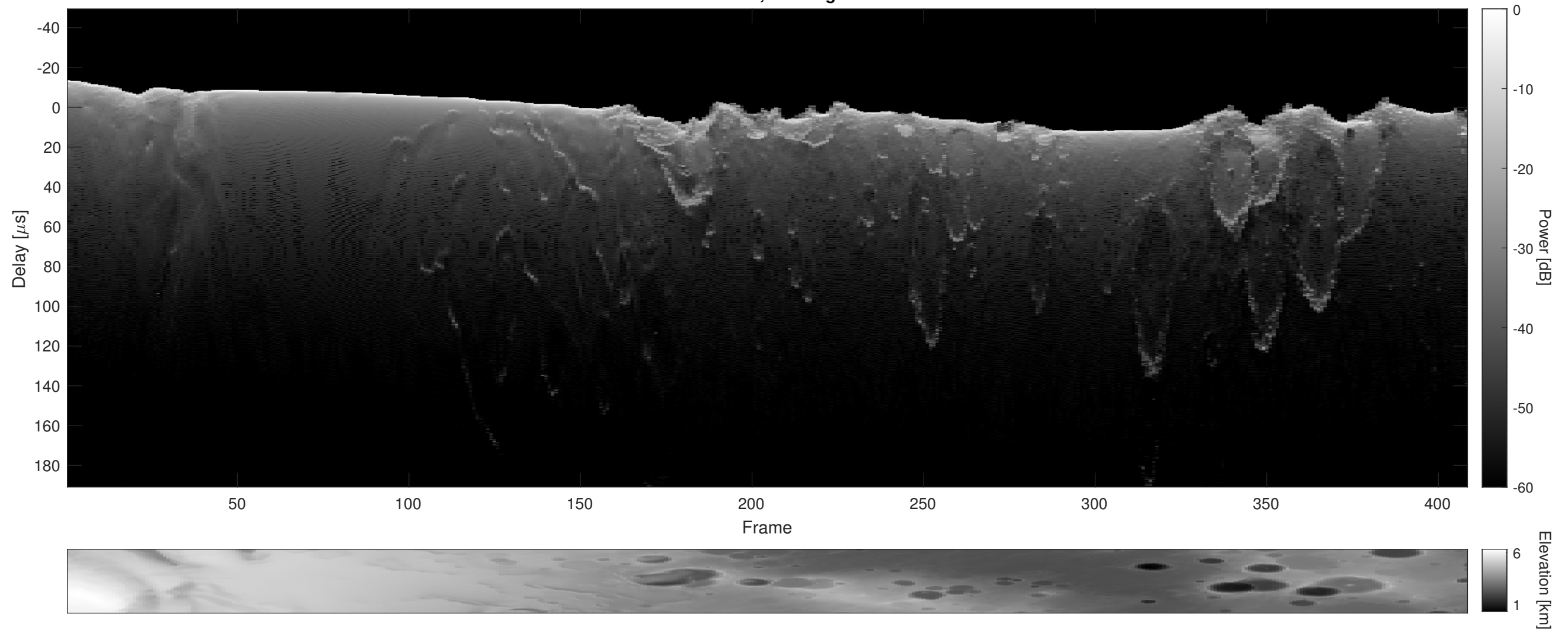
Orbit 16864, Cluttergram
