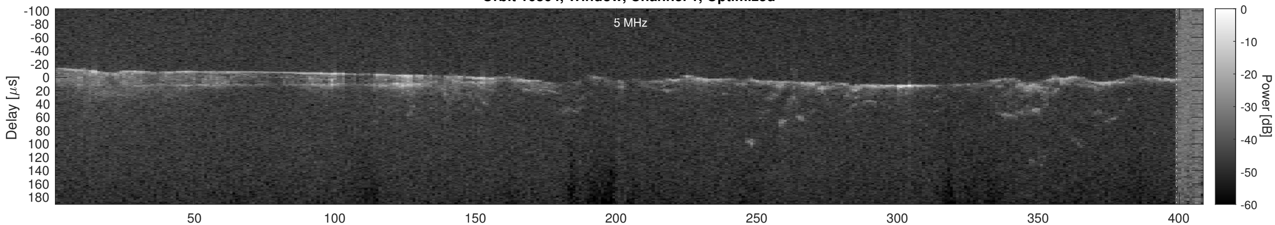
Orbit 16864, Cluttergram
