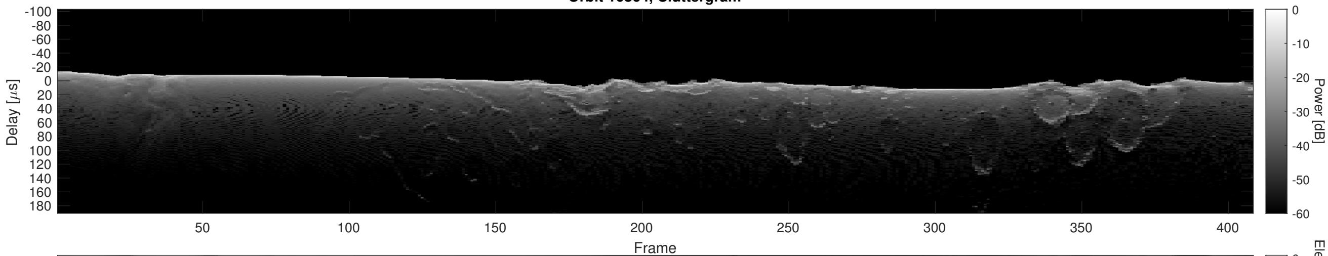
Orbit 16864, Cluttergram
