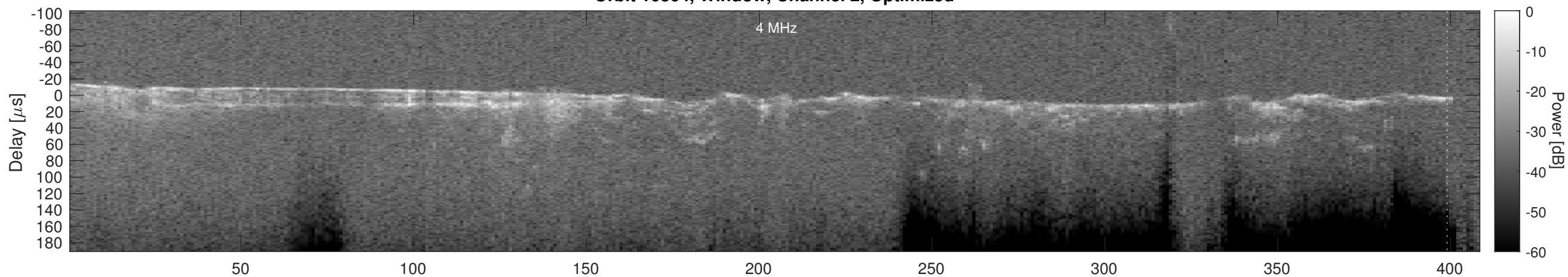
Orbit 16864, Cluttergram
