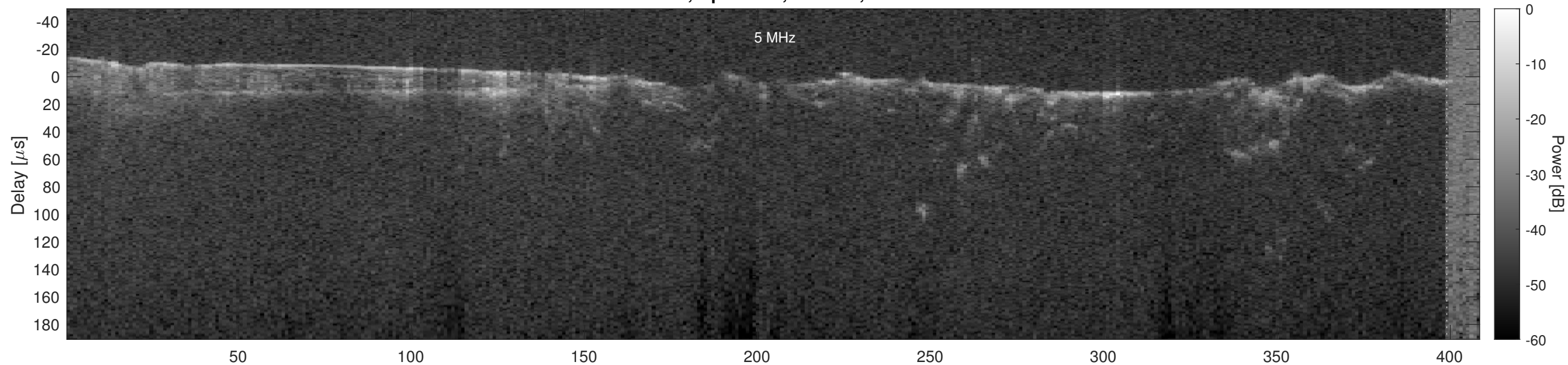
Orbit 16864, Optimized, Window, Channel 2
