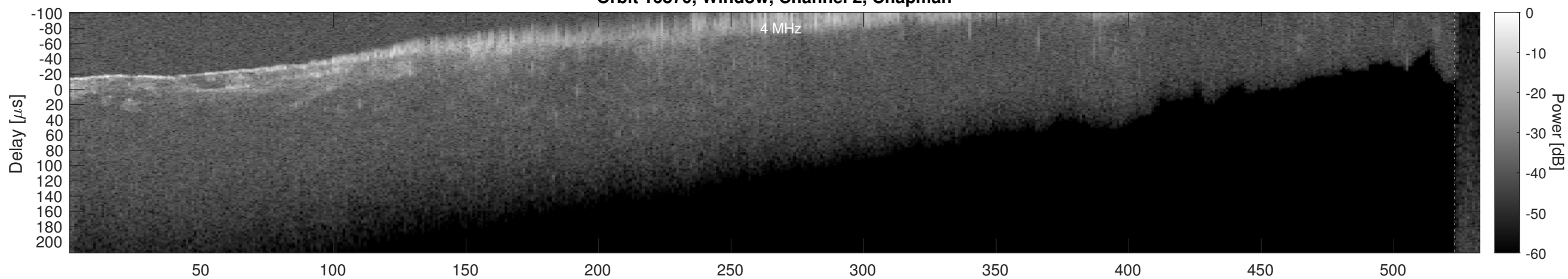
Orbit 16870, Window, Channel 2, Optimized
