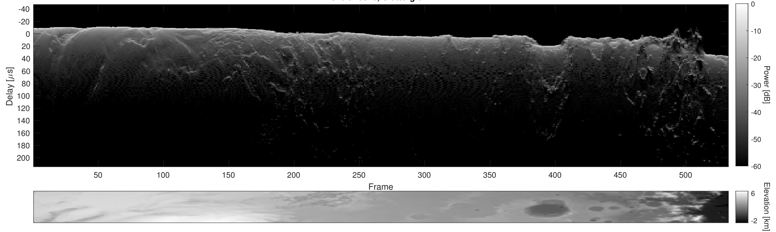
Orbit 16870, Cluttergram
