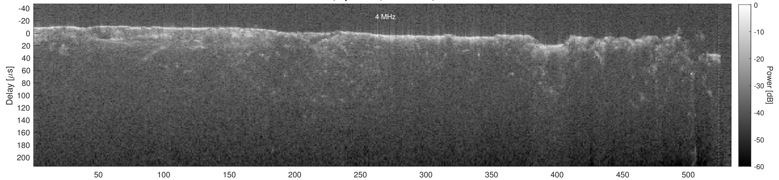
Orbit 16870, Cluttergram
