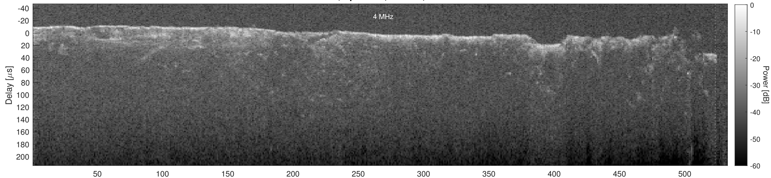
Orbit 16870, Cluttergram
