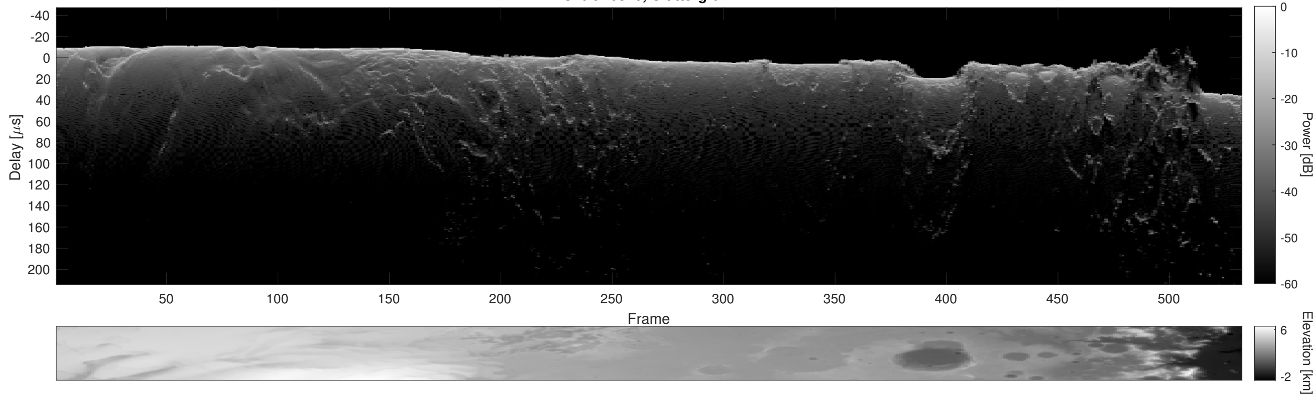
Orbit 16870, Cluttergram
