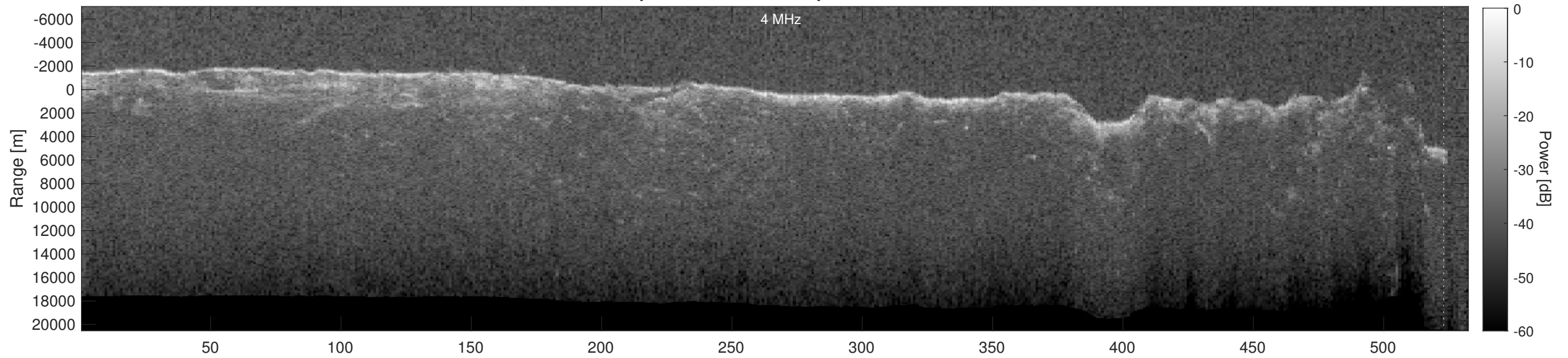
Orbit 16870, Depth-Corrected Cluttergram
