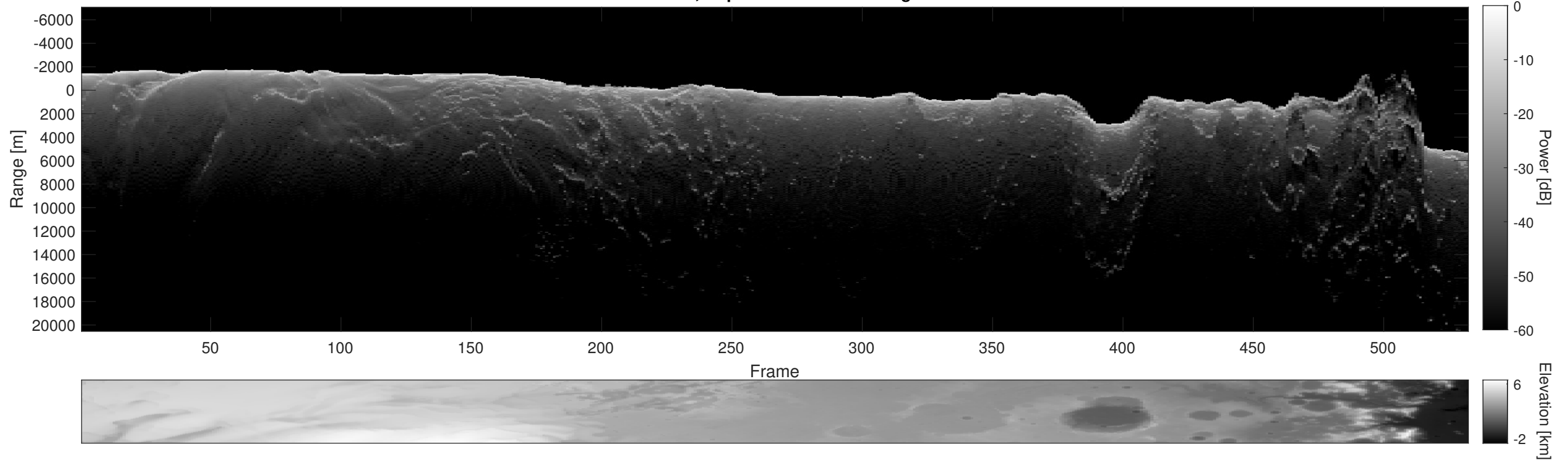
Orbit 16870, Depth-Corrected Cluttergram
