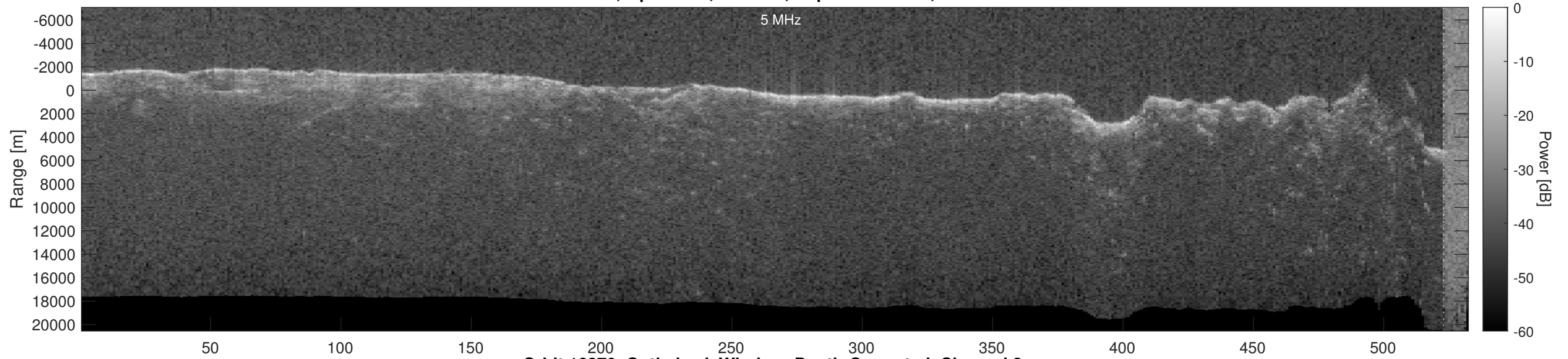
Orbit 16870, Optimized, Window, Depth-Corrected, Channel 2
