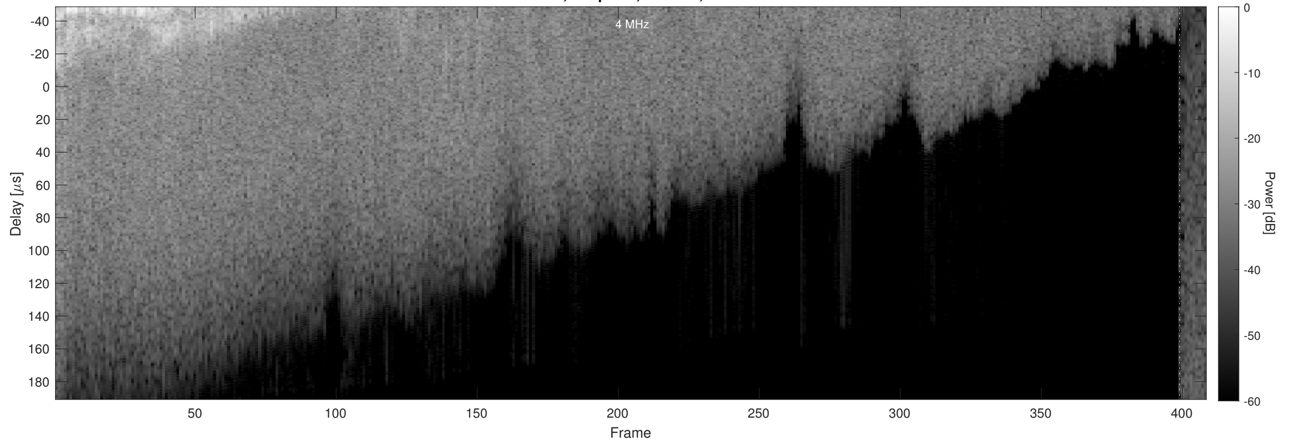
Orbit 16871, Chapman, Window, Channel 2
