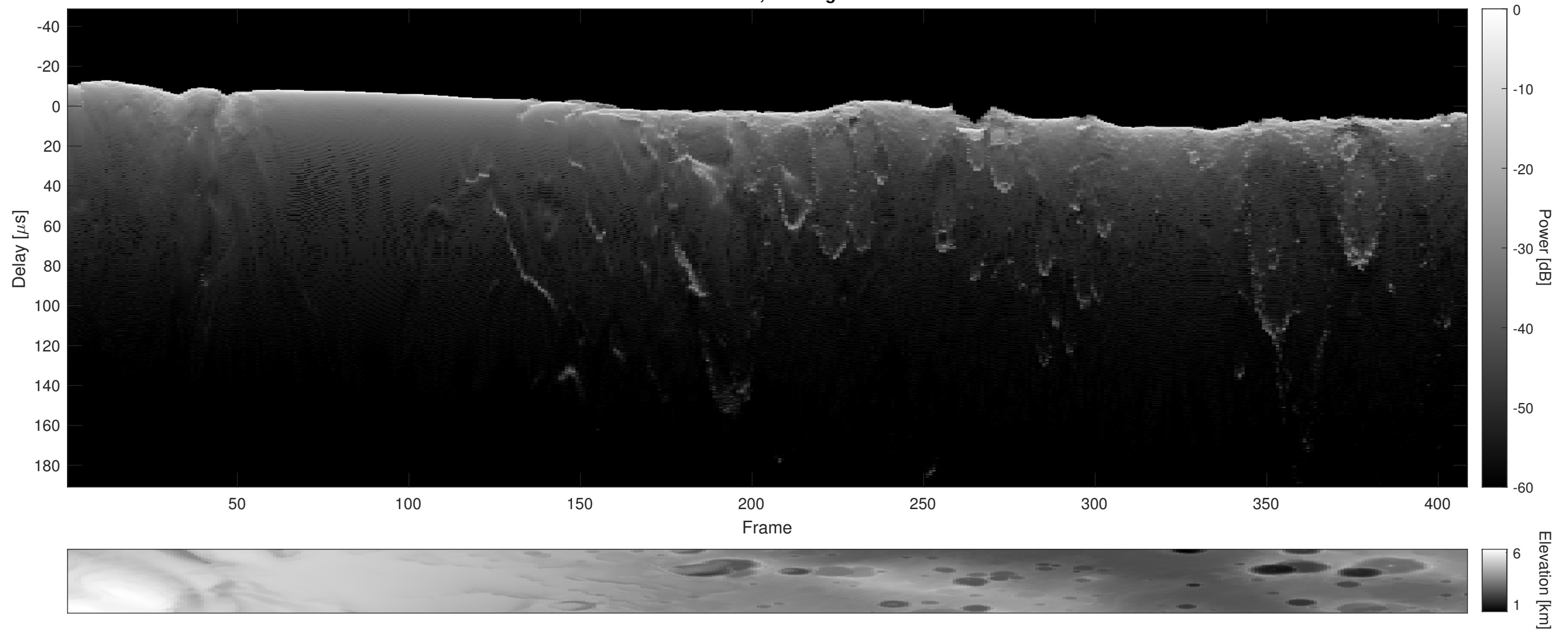
Orbit 16871, Cluttergram
