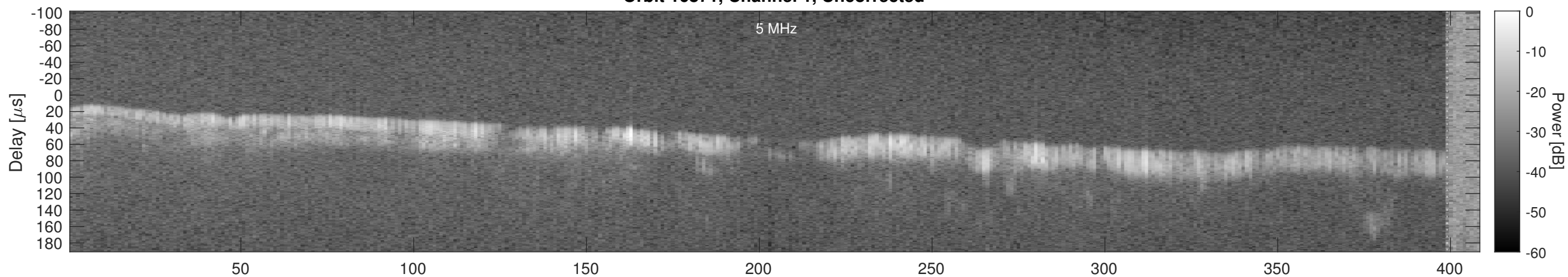
Orbit 16871, Window, Channel 1, Chapman
