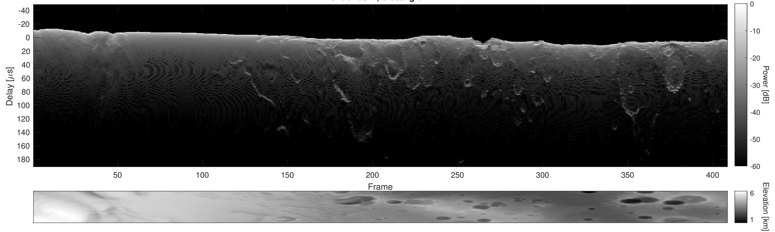
Orbit 16871, Cluttergram
