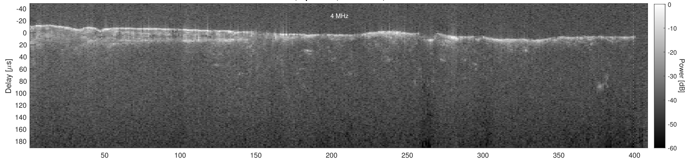
Orbit 16871, Cluttergram
