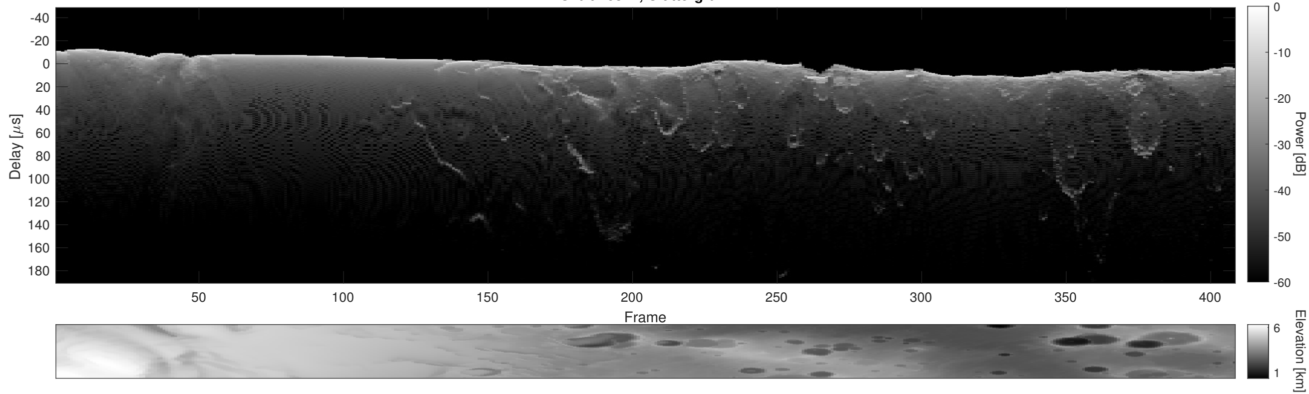
Orbit 16871, Cluttergram
