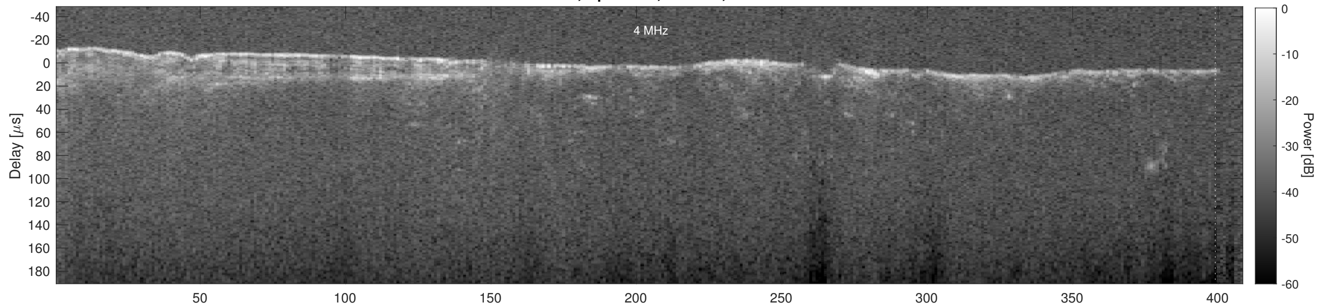
Orbit 16871, Cluttergram
