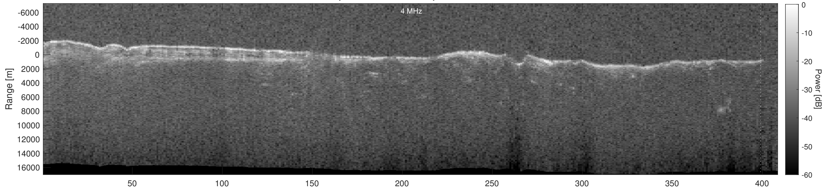
Orbit 16871, Depth-Corrected Cluttergram
