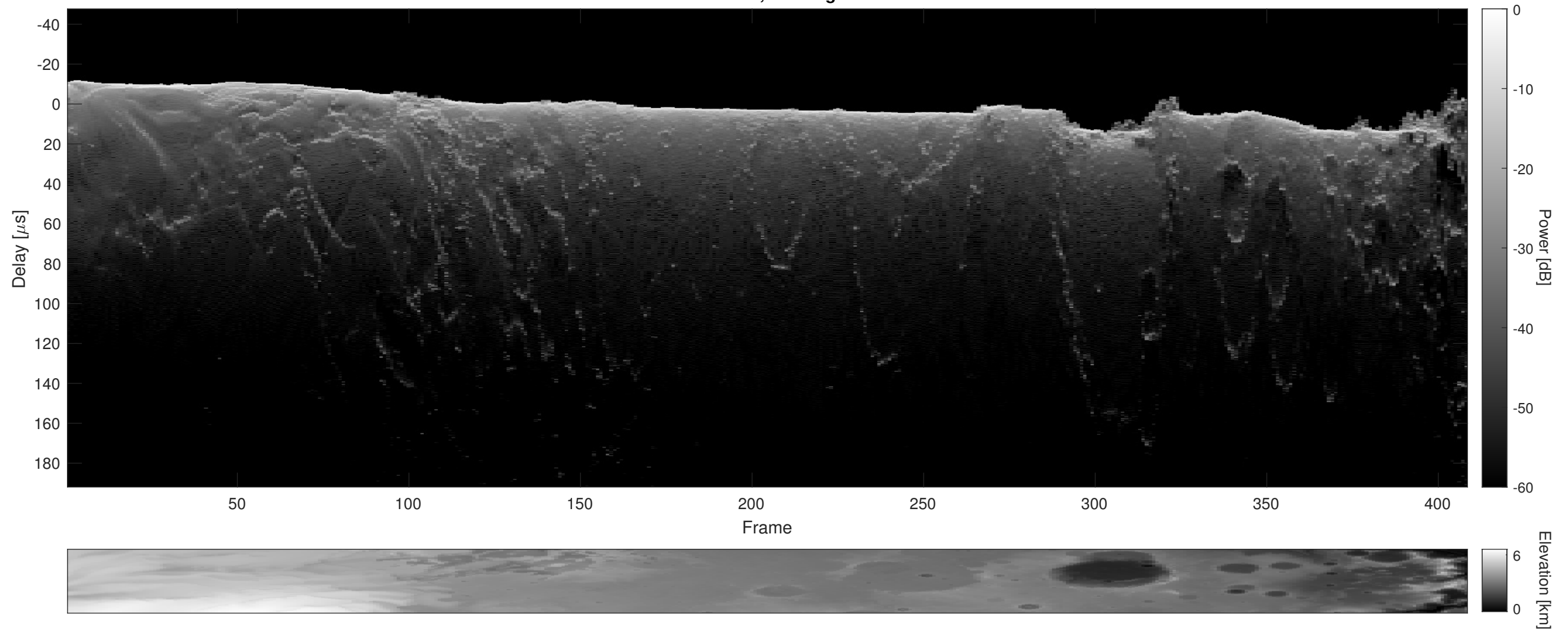
Orbit 16877, Cluttergram
