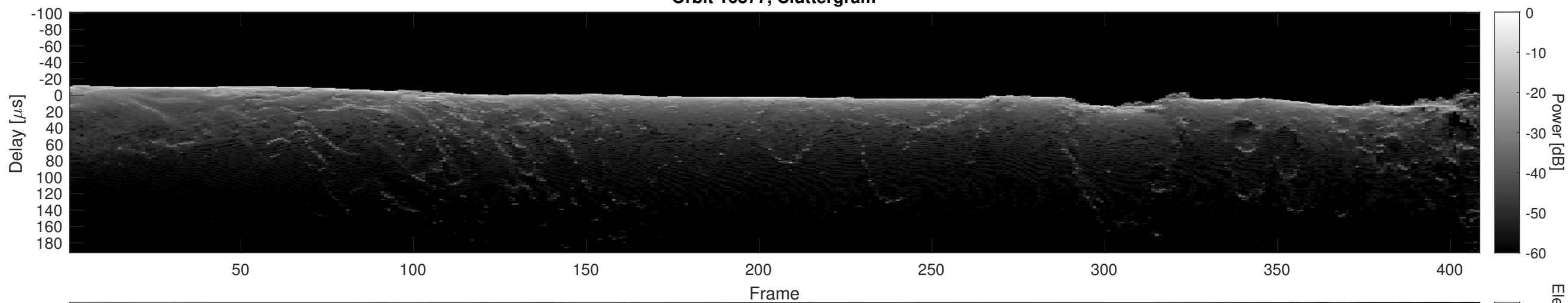
Orbit 16877, Cluttergram
