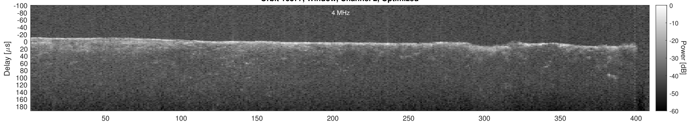
Orbit 16877, Cluttergram
