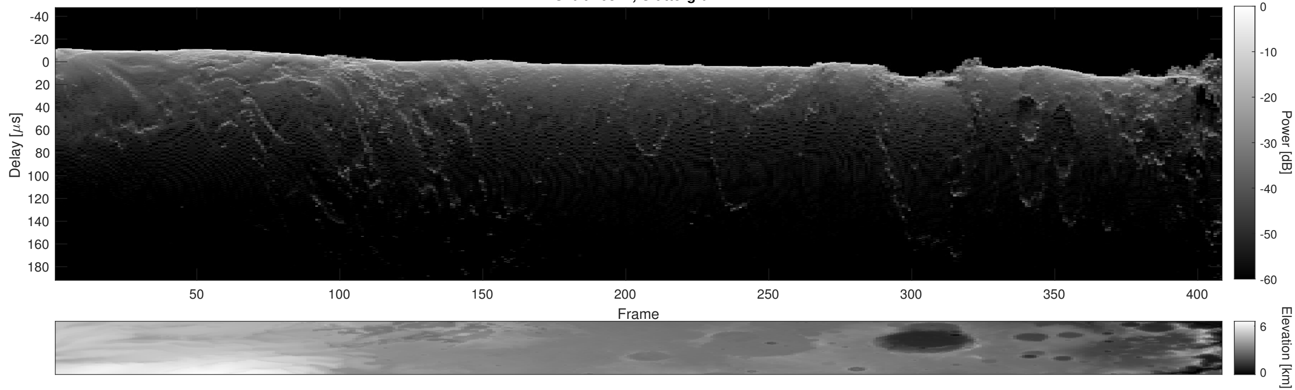
Orbit 16877, Cluttergram
