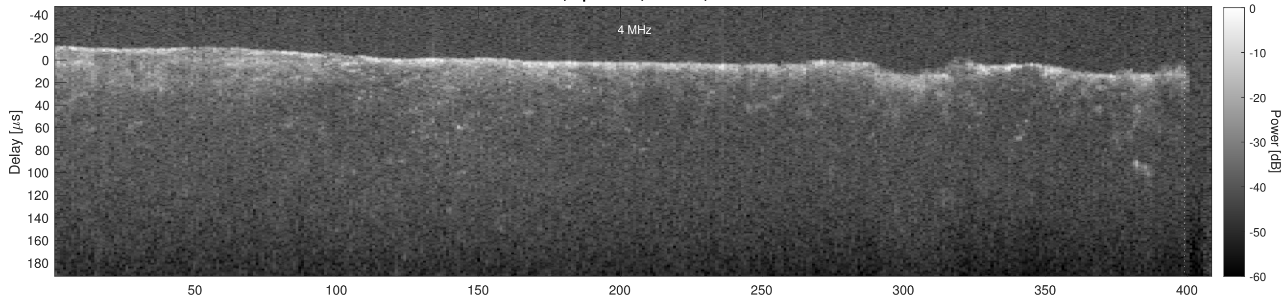
Orbit 16877, Cluttergram
