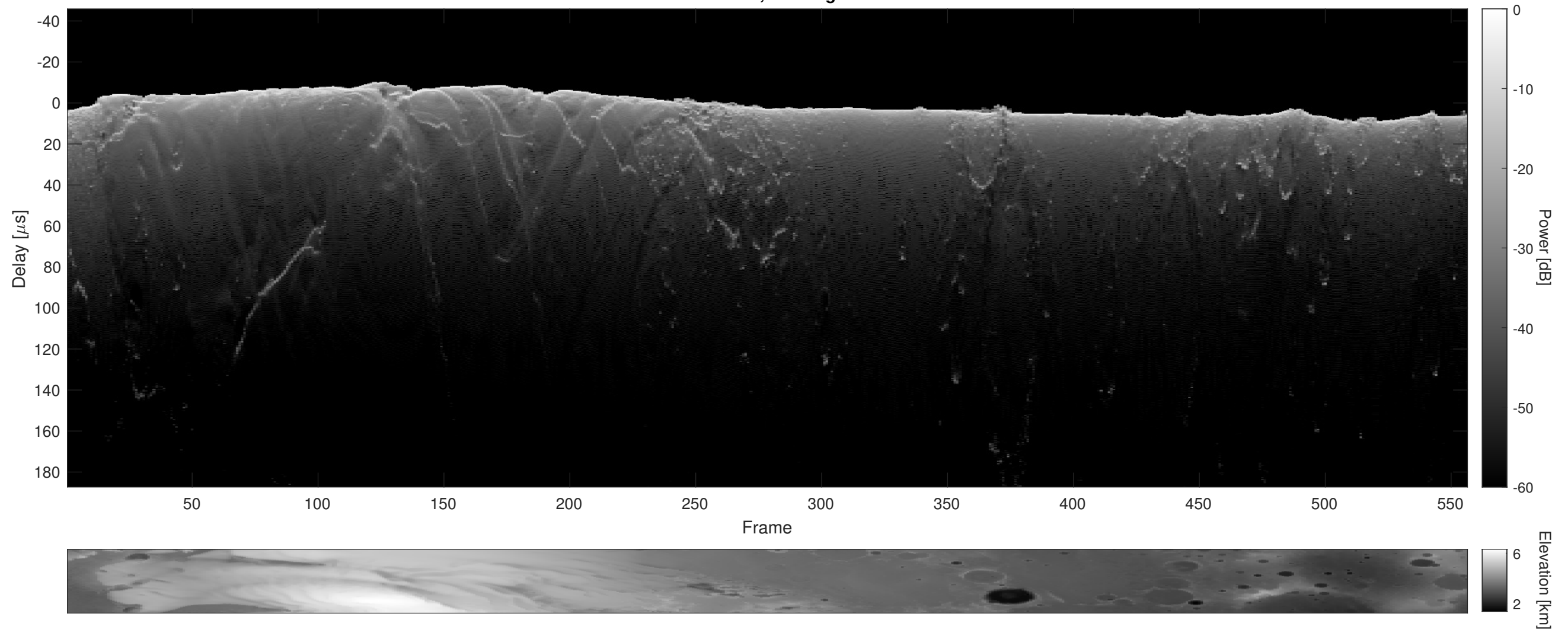
Orbit 16881, Cluttergram
