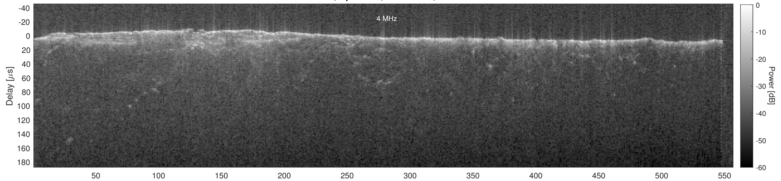
Orbit 16881, Cluttergram
