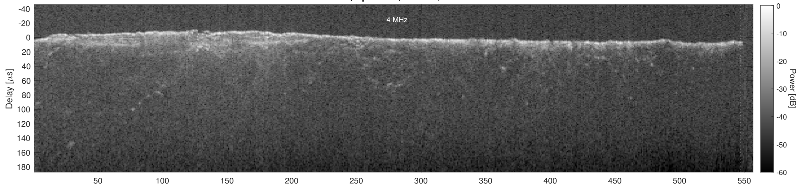
Orbit 16881, Cluttergram
