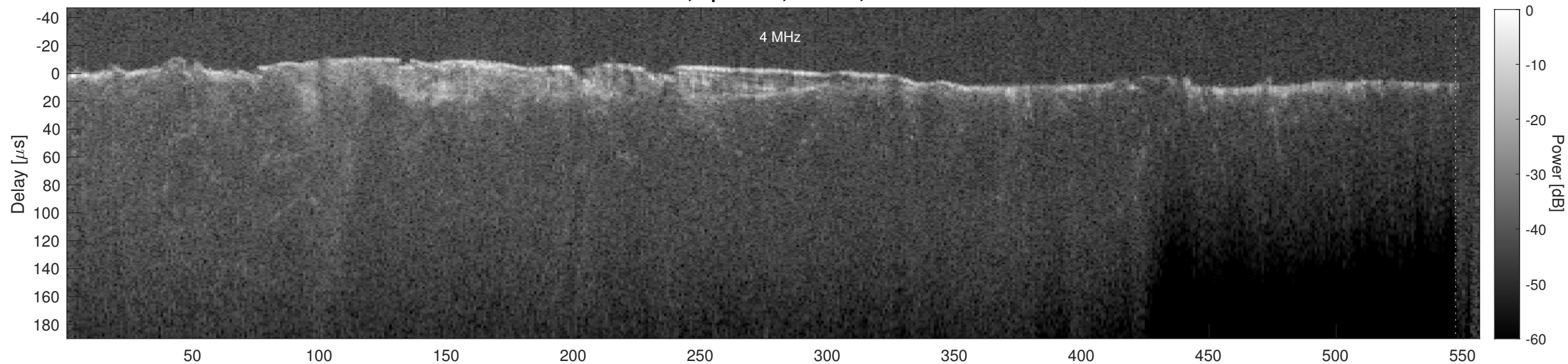
Orbit 16882, Cluttergram
