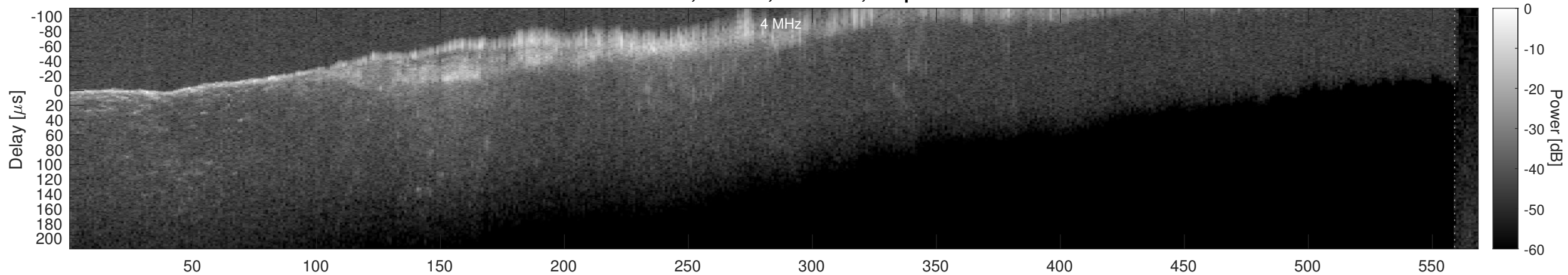
Orbit 16890, Window, Channel 2, Optimized
