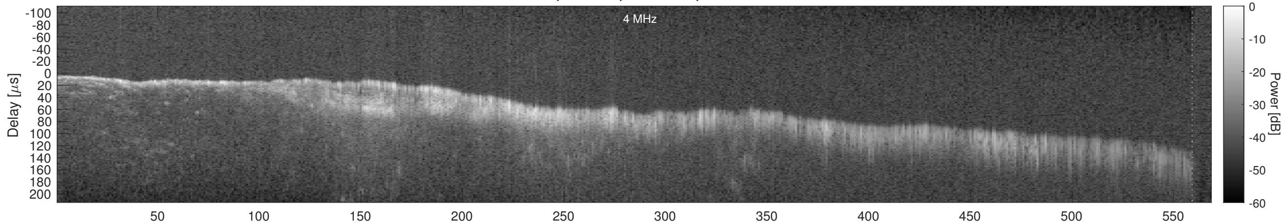
Orbit 16890, Window, Channel 2, Chapman
