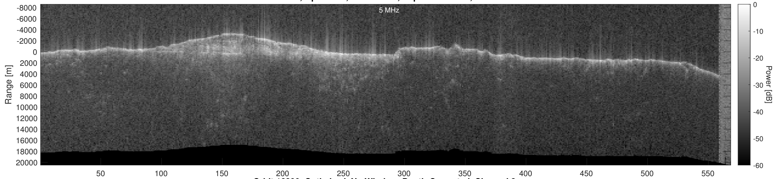
Orbit 16890, Optimized, No Window, Depth-Corrected, Channel 2
