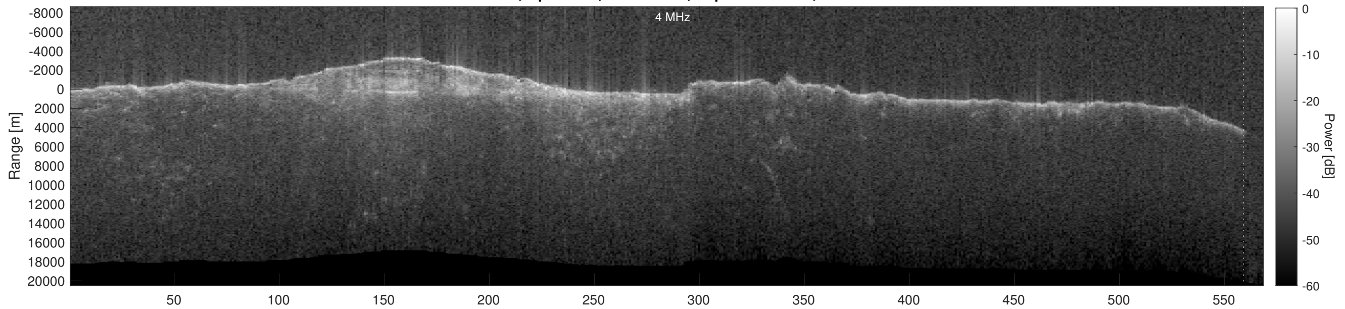
Orbit 16890, Depth-Corrected Cluttergram
