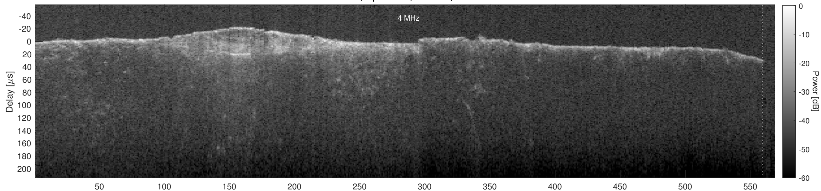
Orbit 16890, Cluttergram
