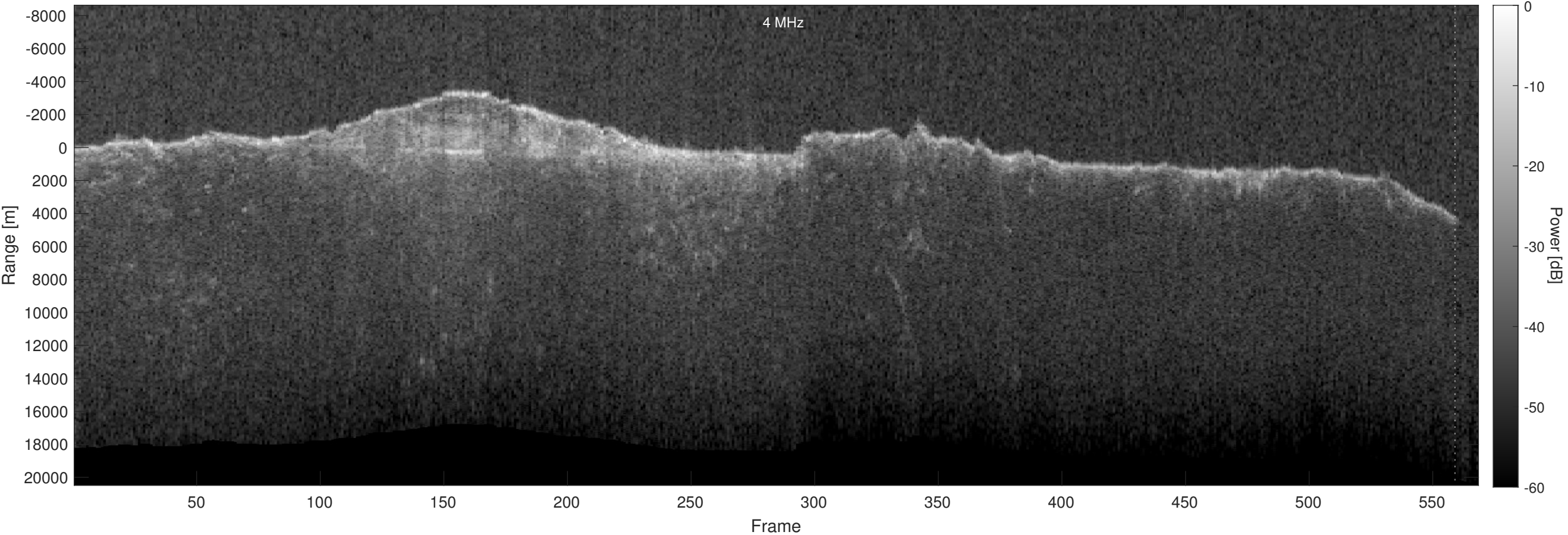
Orbit 16890, Optimized, Window, Depth-Corrected, Channel 2
