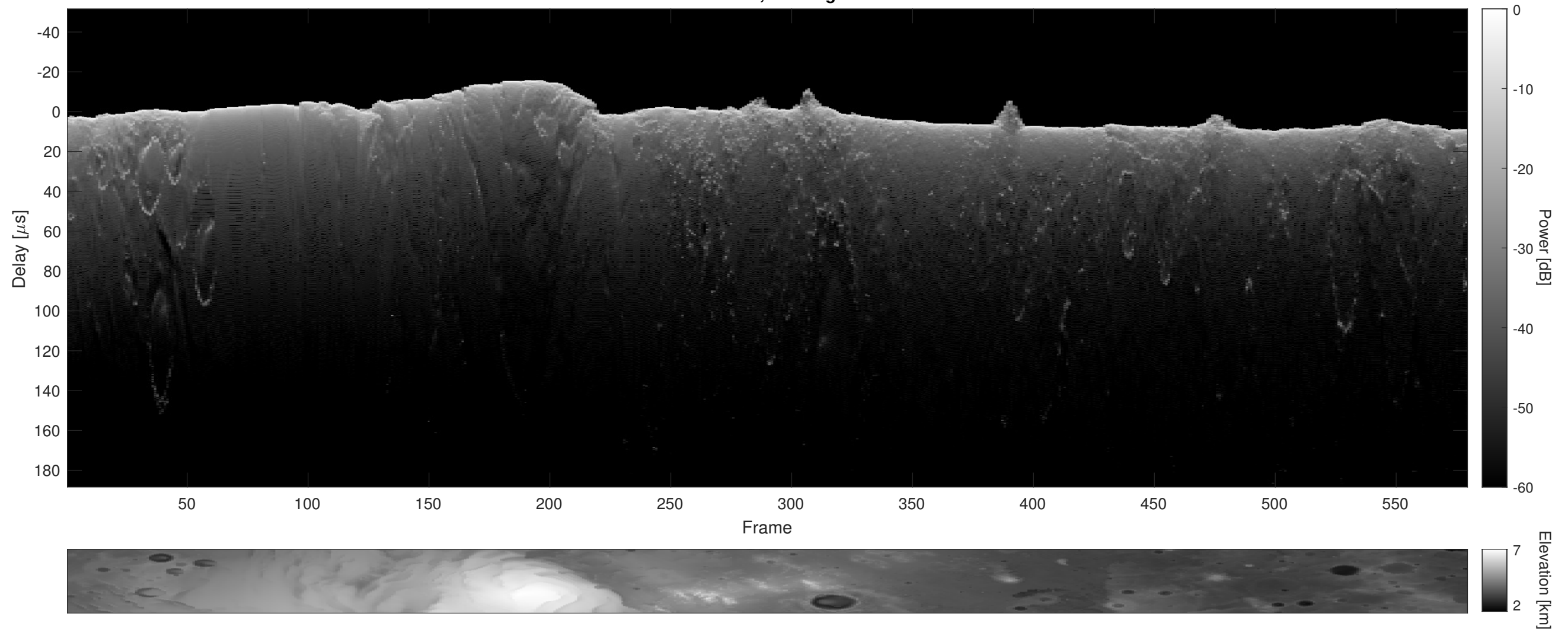
Orbit 16894, Cluttergram
