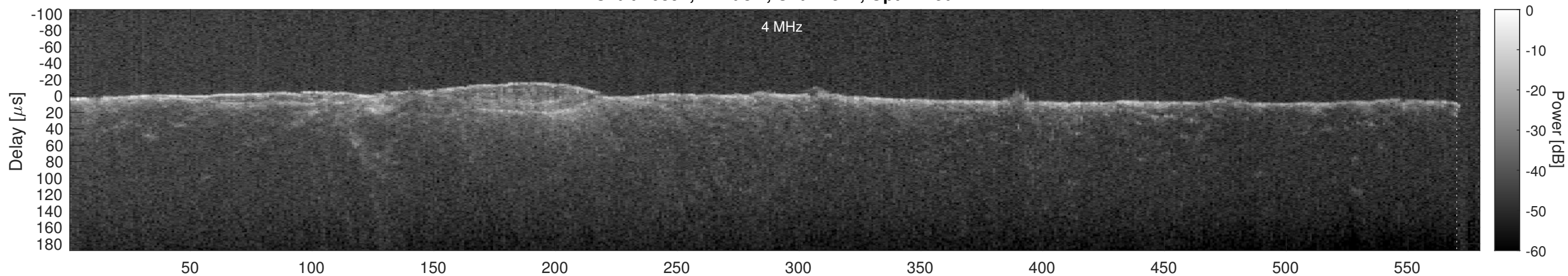
Orbit 16894, Cluttergram
