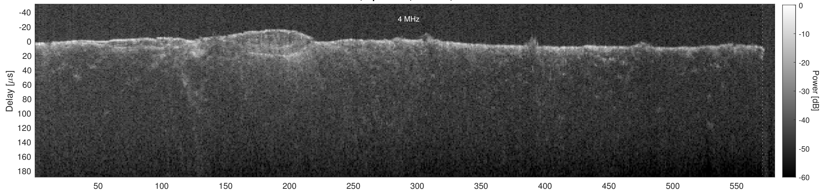
Orbit 16894, Cluttergram
