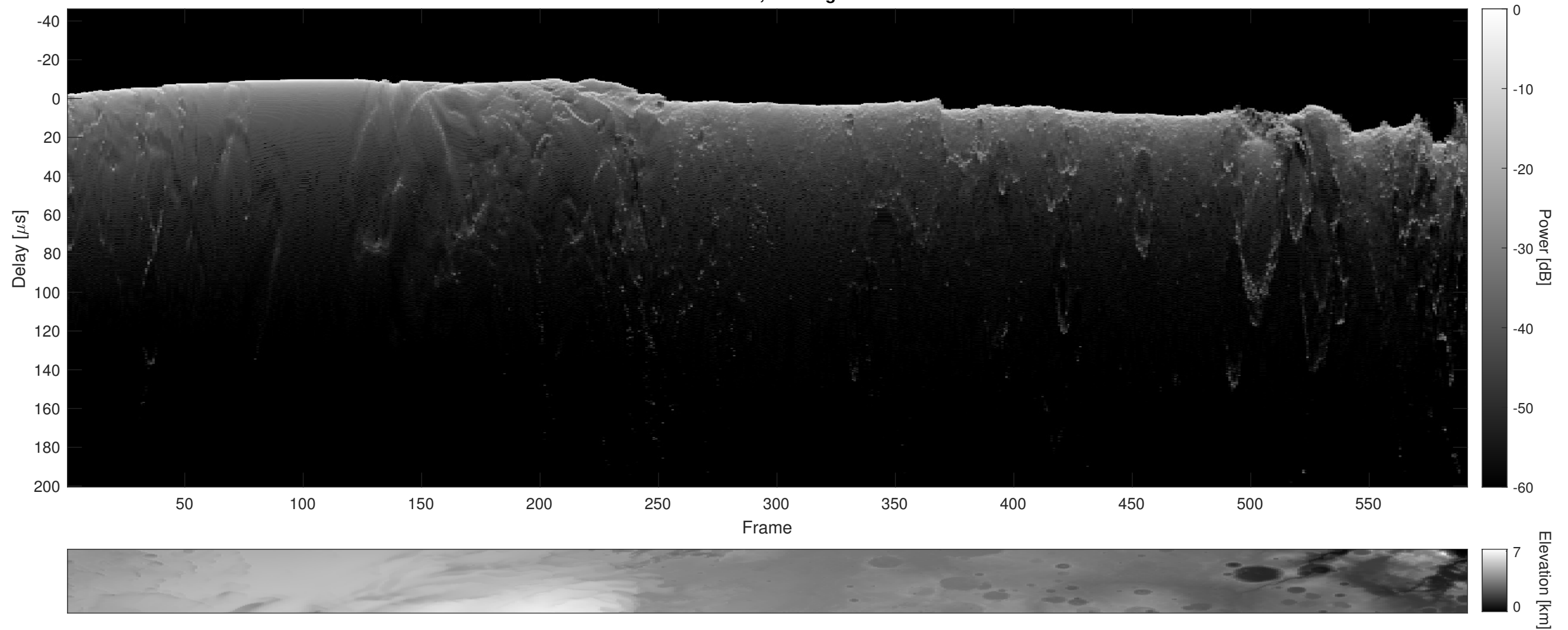
Orbit 16898, Cluttergram
