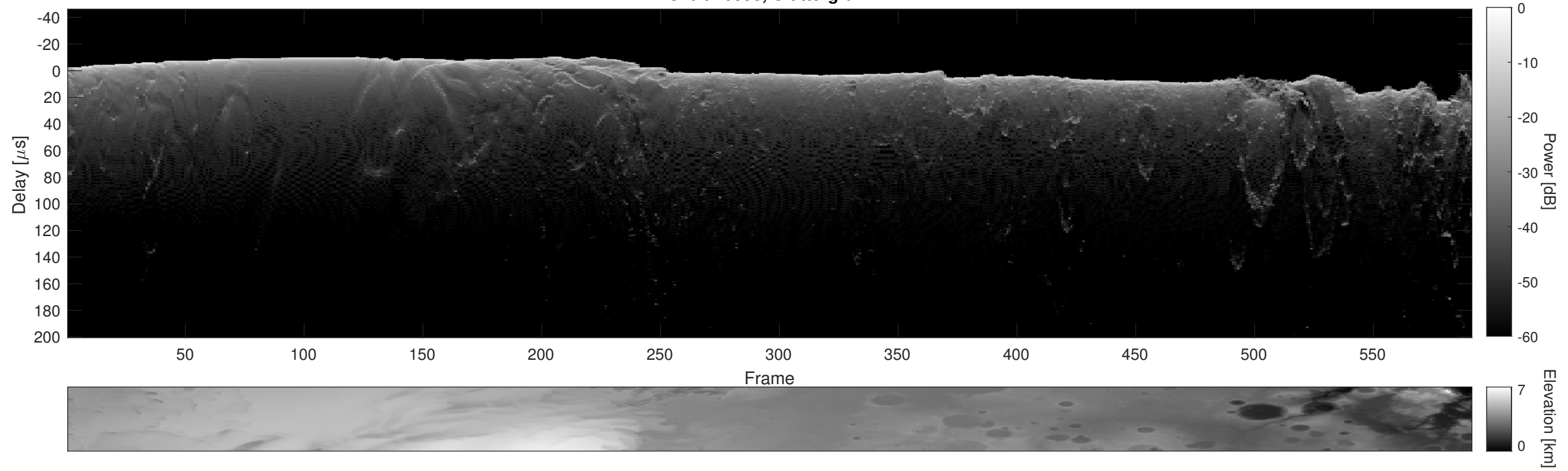
Orbit 16898, Cluttergram
