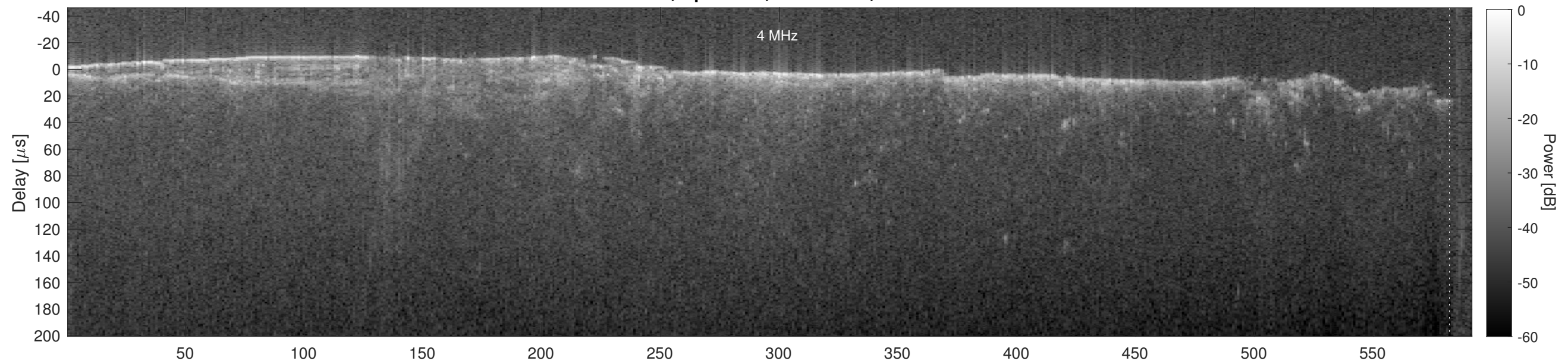
Orbit 16898, Cluttergram
