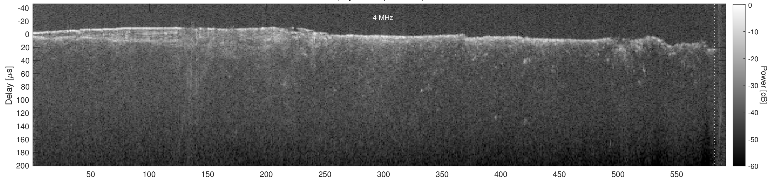
Orbit 16898, Cluttergram
