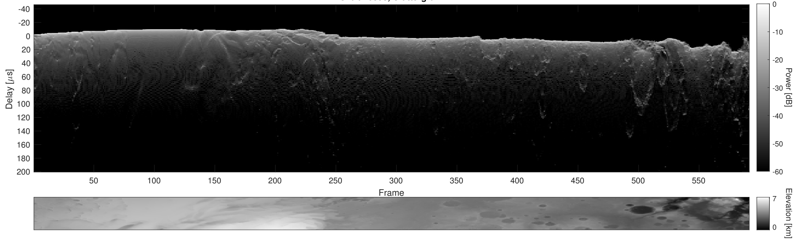
Orbit 16898, Cluttergram
