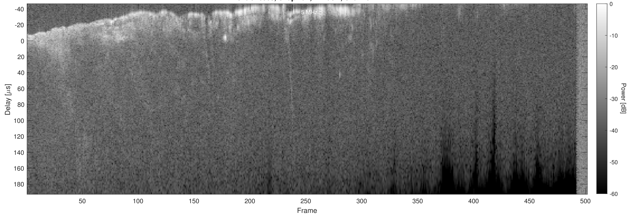
Orbit 16903, Chapman, Window, Channel 2
