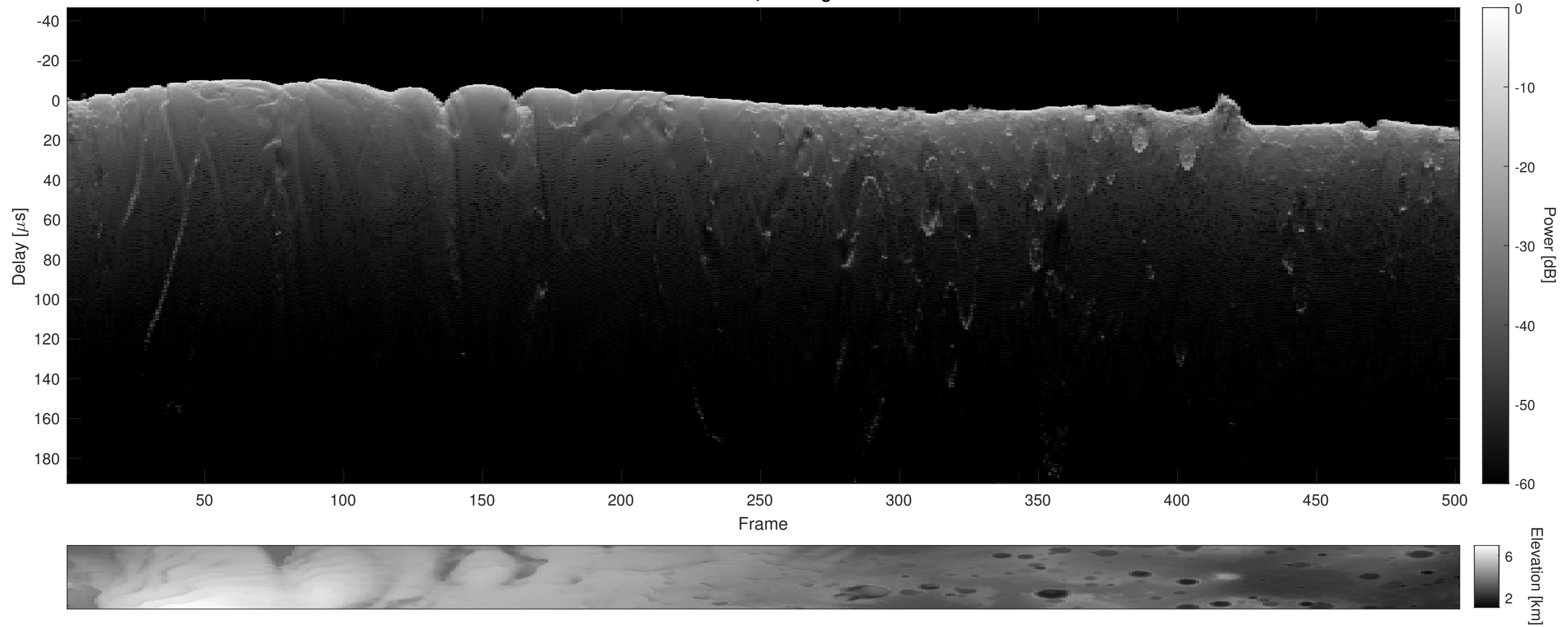
Orbit 16903, Cluttergram
