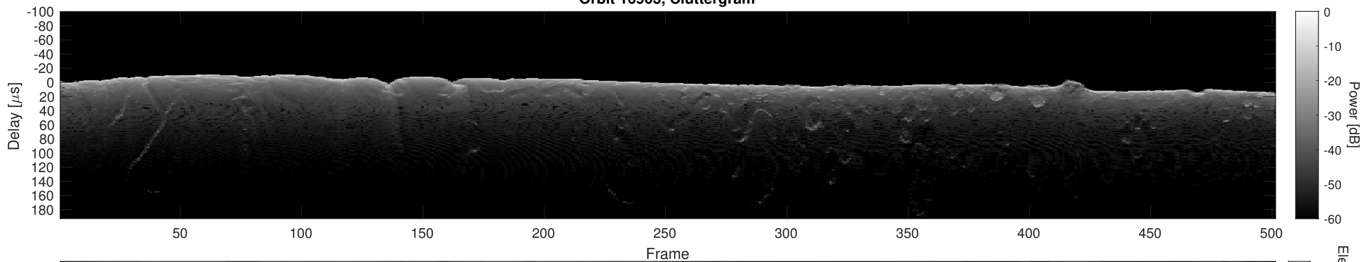
Orbit 16903, Cluttergram
