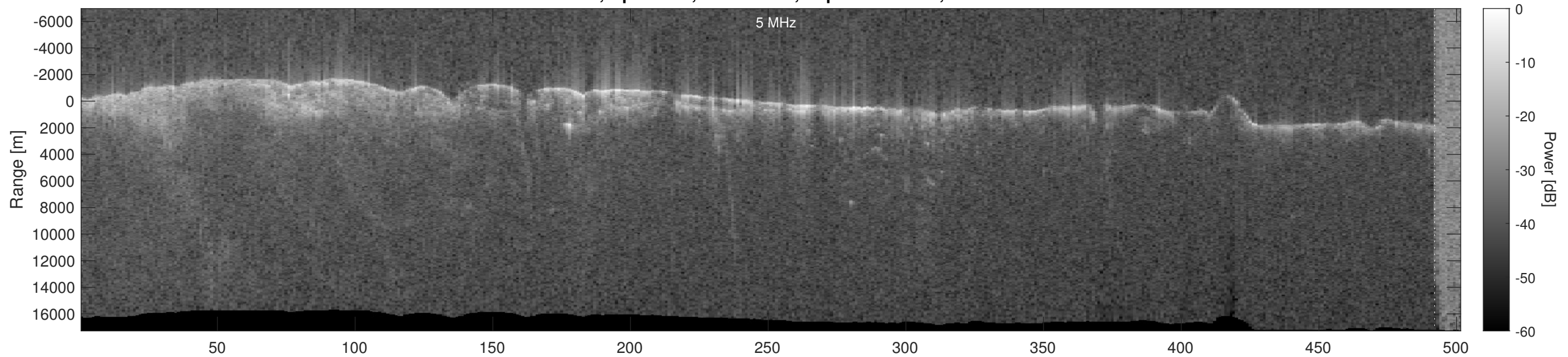
Orbit 16903, Optimized, No Window, Depth-Corrected, Channel 2
