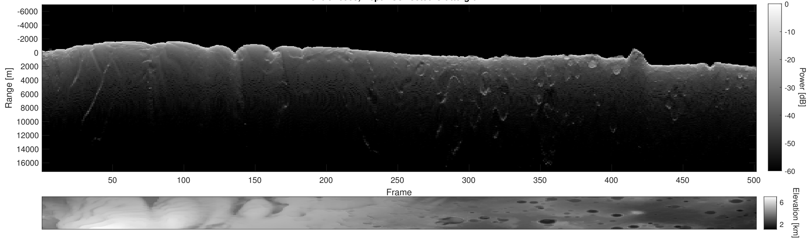
Orbit 16903, Depth-Corrected Cluttergram
