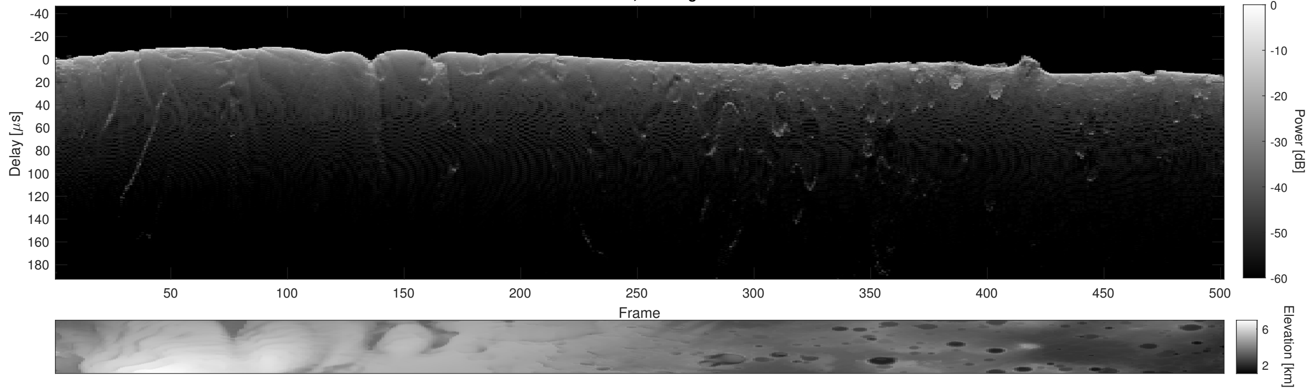
Orbit 16903, Cluttergram
