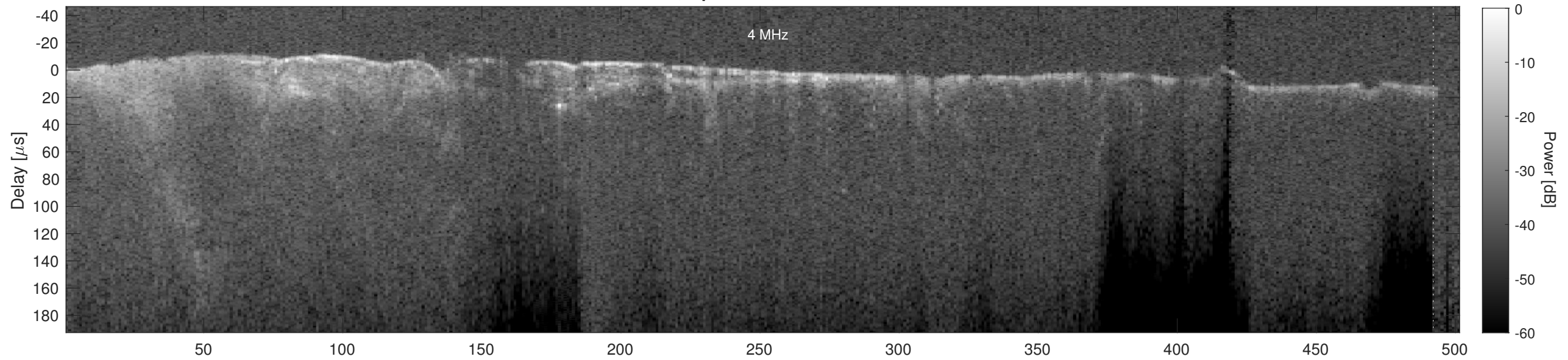
Orbit 16903, Cluttergram
