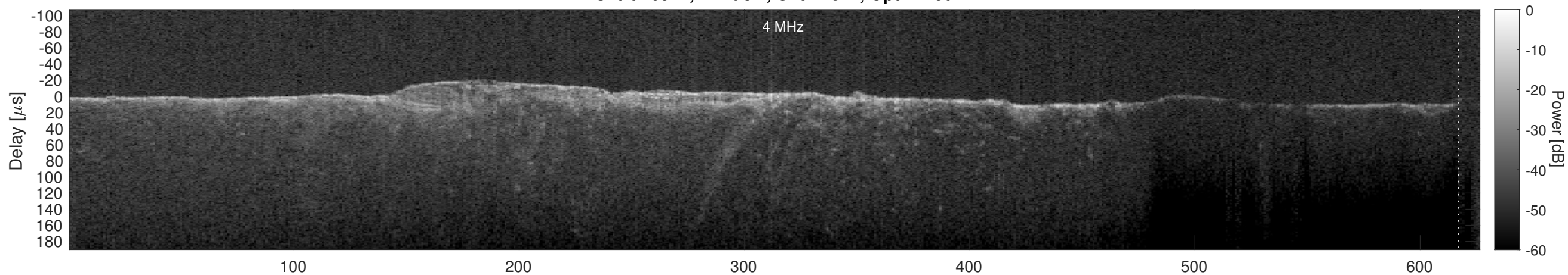
Orbit 16914, Cluttergram
