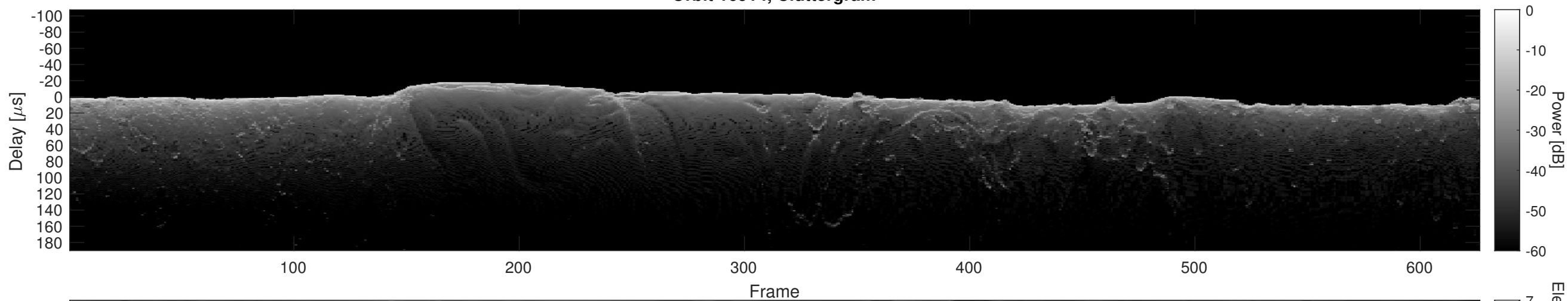
Orbit 16914, Cluttergram
