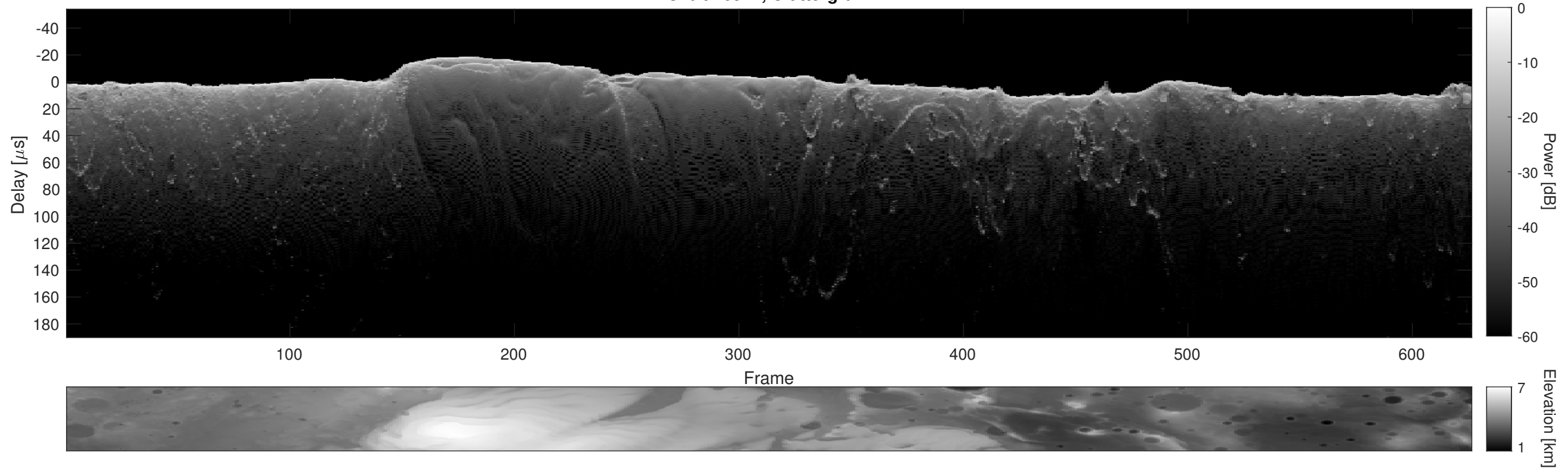
Orbit 16914, Cluttergram
