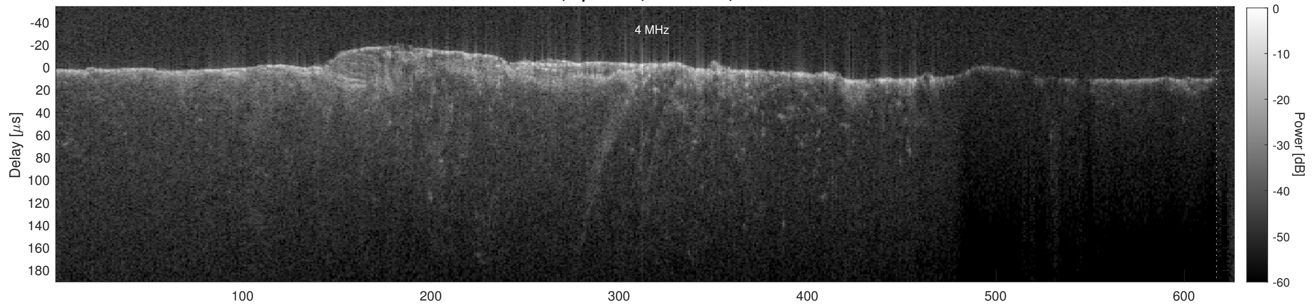
Orbit 16914, Cluttergram
